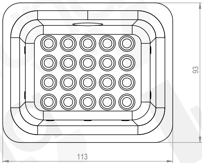
VISTA INFERIORE (bottom View)
