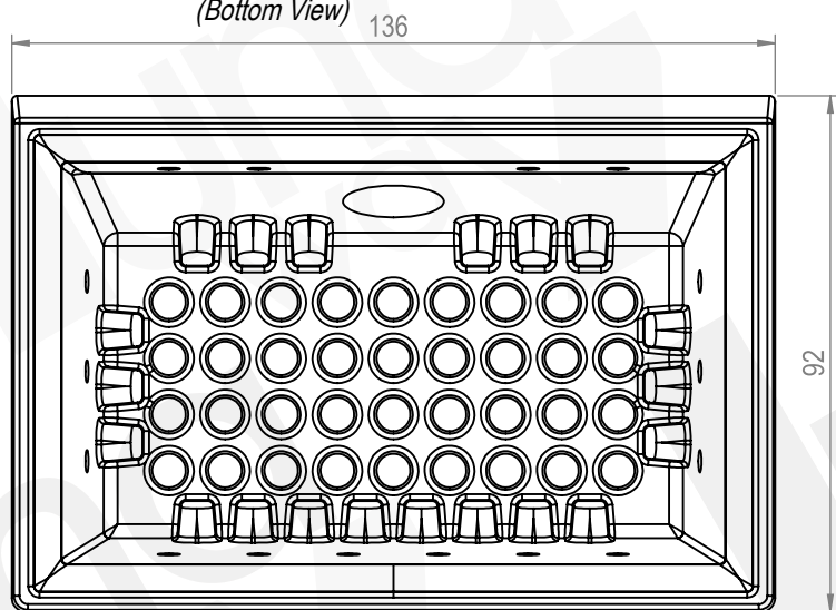
VISTA INFERIORE (Bottom View)
