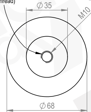
filettatura sinistrorsa (left hand thread)
