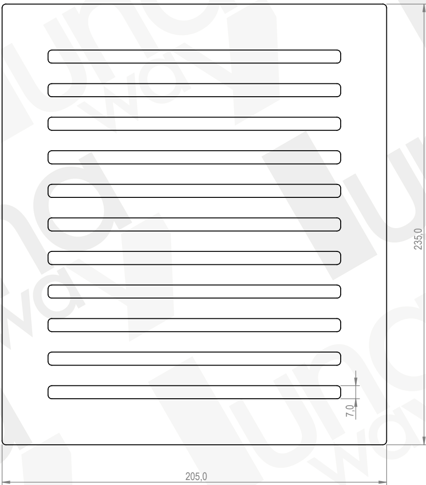
VISTA FRONTALE (frontal view)
